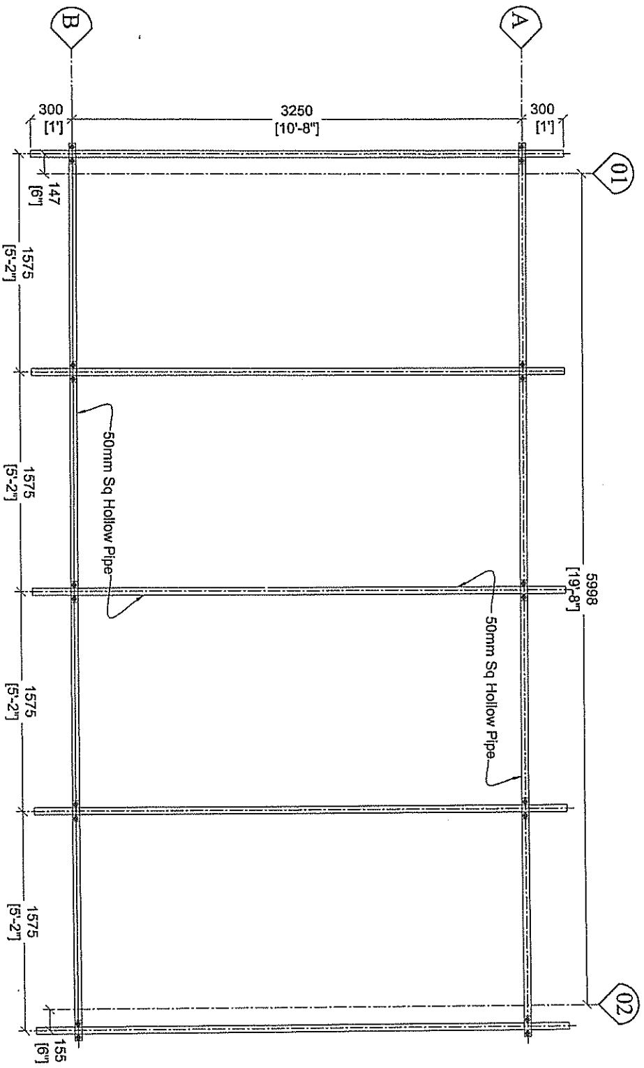
ROOF PLAN
